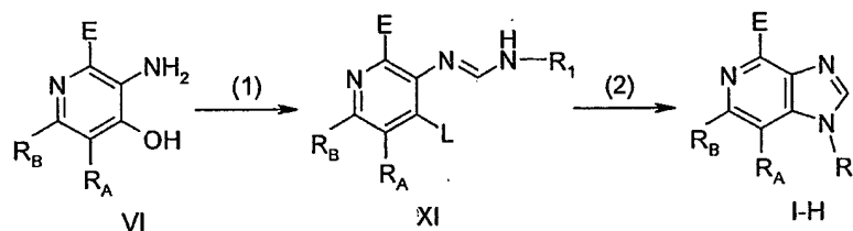
Reaction Scheme IX
